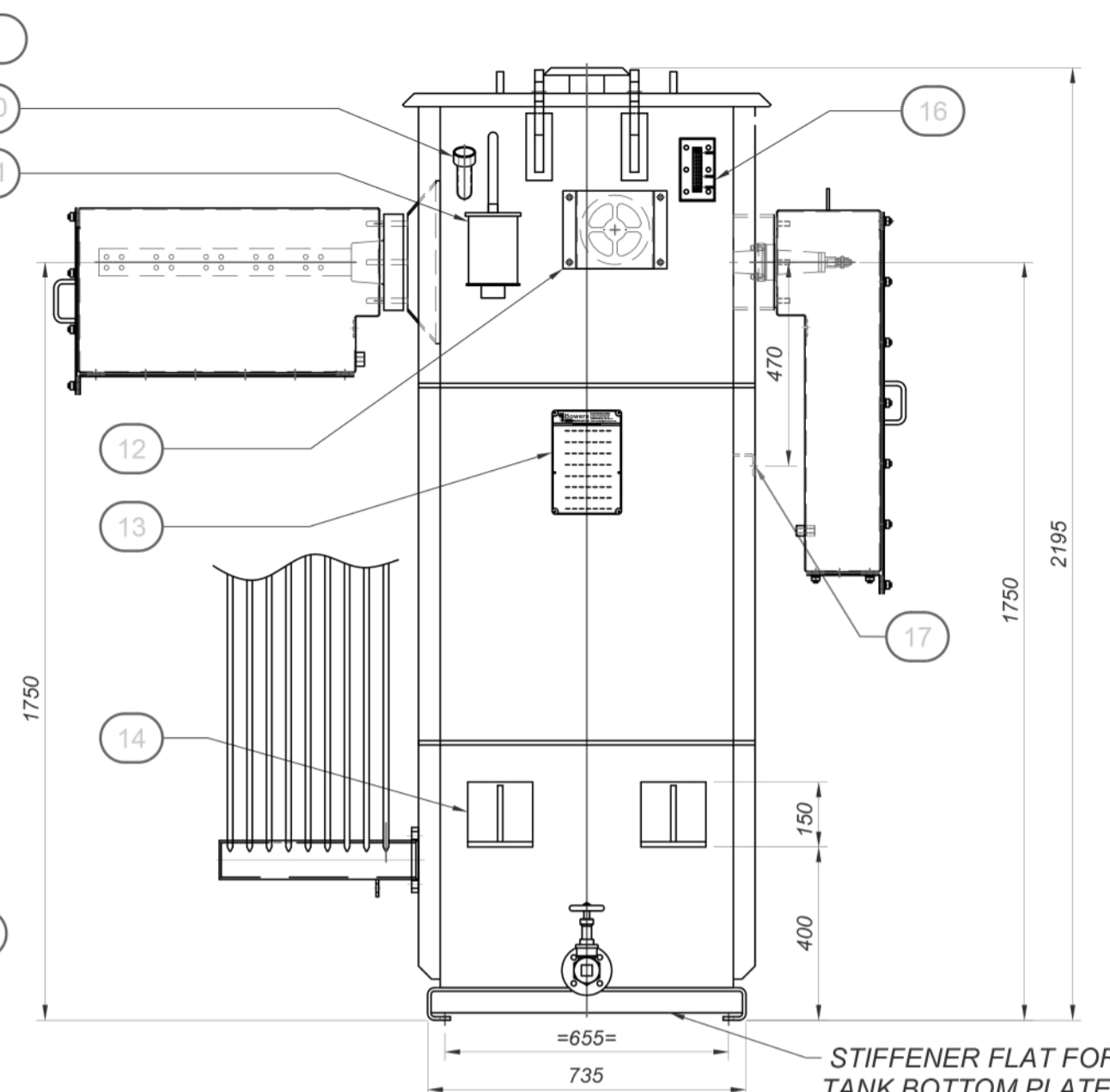
SIDE VIEW
