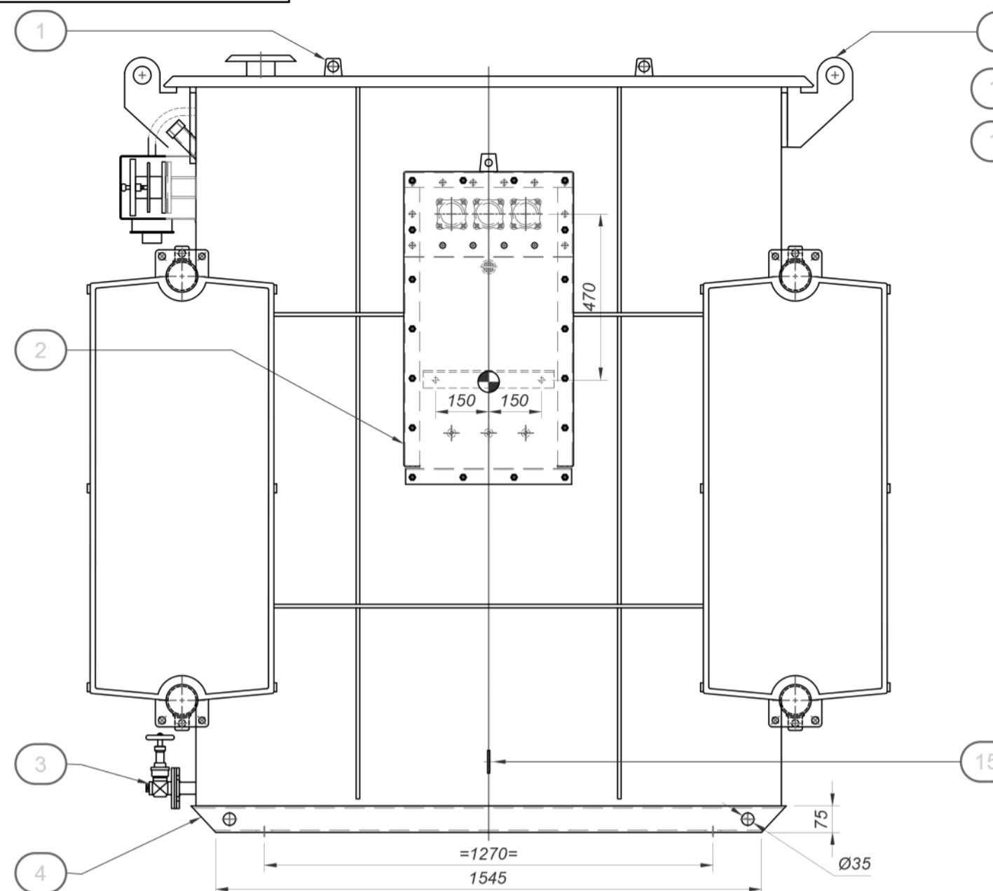
FRONT VIEW
